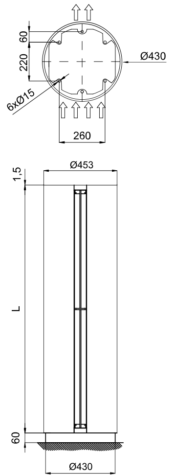
Floor fixing points with foot
